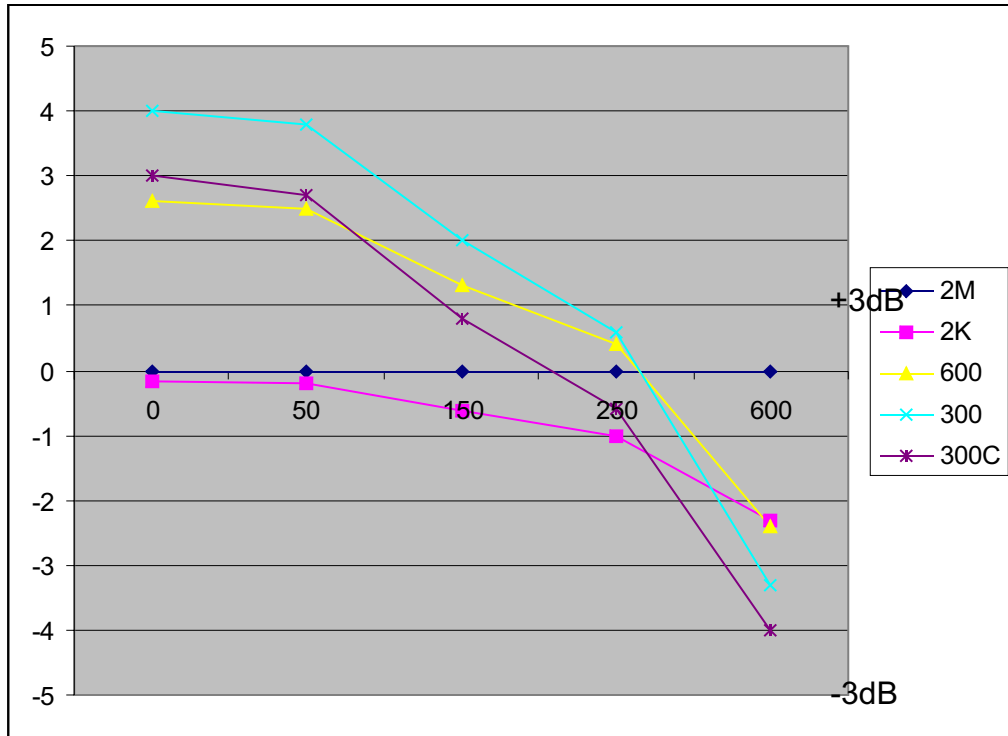
MicrophoneOutputImpedance
