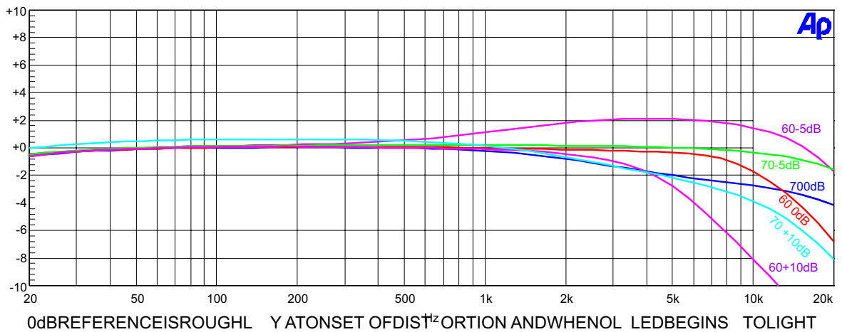
60s-70sSWITCHFREQUENCY RESPONSE ATVARIOUSGAINS&COMPENSA TEDwith TRIMPOT
