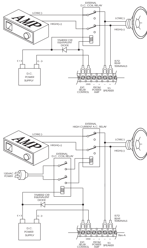
Figure 7-4 Using the External Relay connections.
