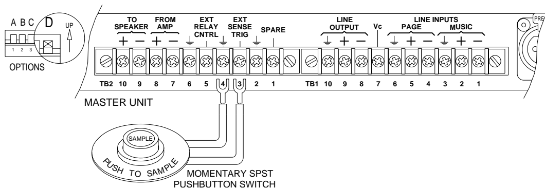
Figure Appendix A-1. Using option switch D and a remote momentary pushbutton for externally controlled sampling.
