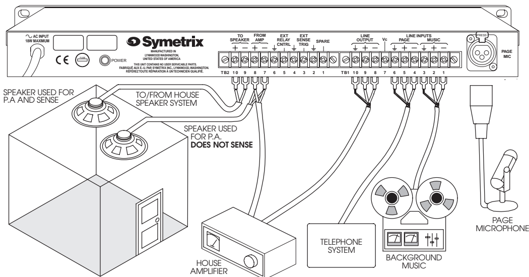
Figure 3-1. 572 generic hookup diagram.
