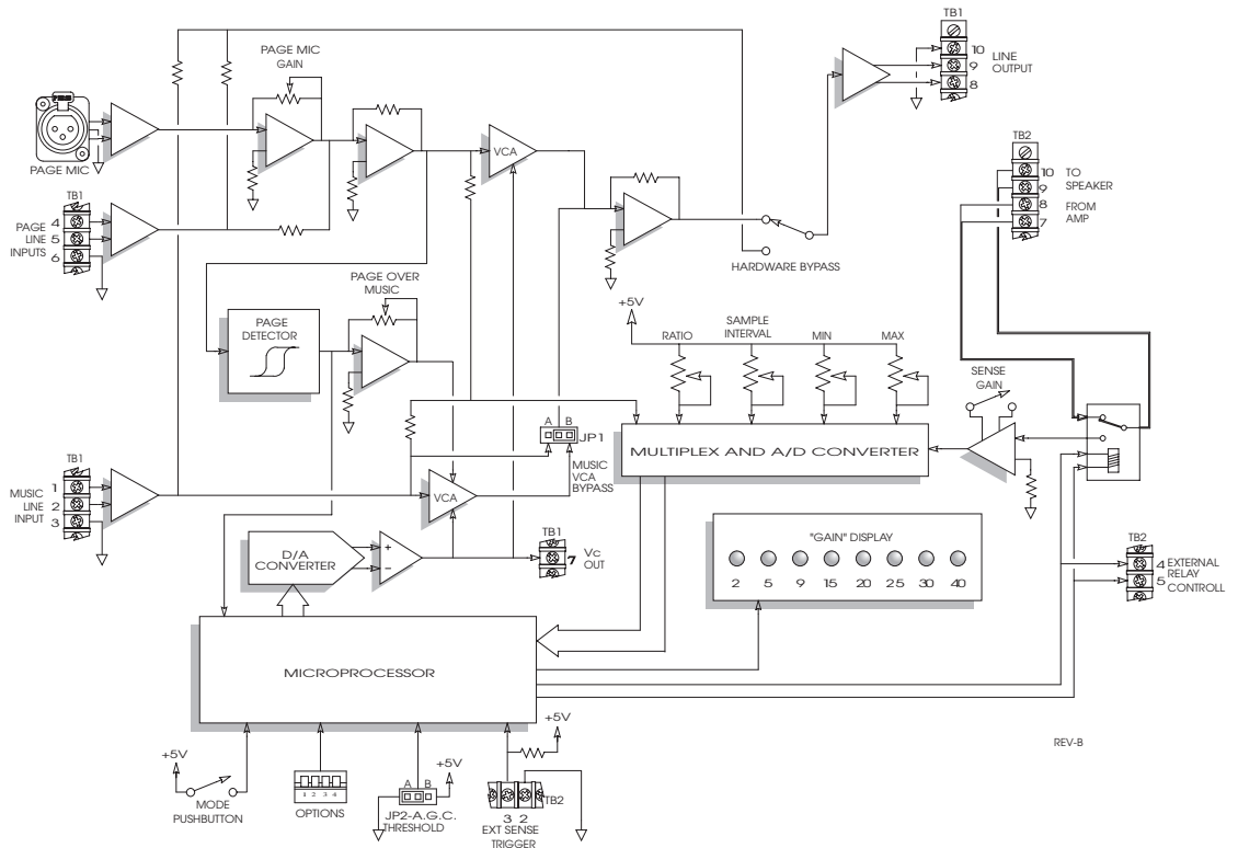
Figure 7-1. 572 Block Diagram.
