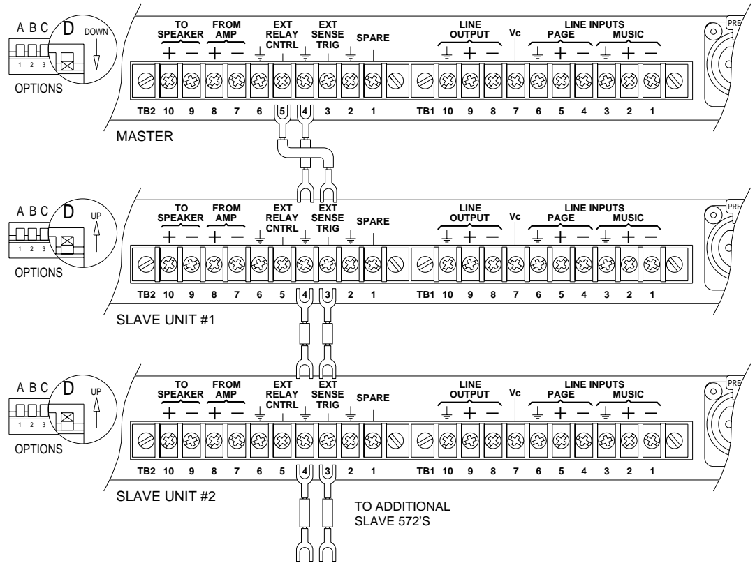
Figure Appendix A-2. Multiple 572 master-slave connections for simultaneous sampling.
